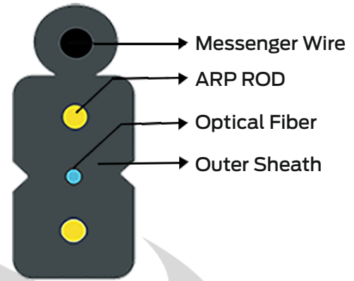
FIG. 8 OUTDOOR DROP
