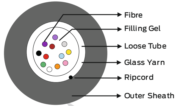
UNARMoured WITH GLASS YARN
