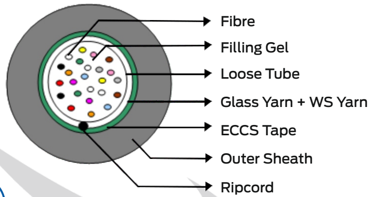
UNITUBE ARMoured WITH GLASS YARNS
