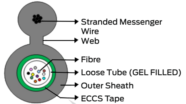
ARMOURED UNITUBE FIG 8
