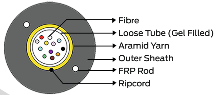
UNITUBE SINGLE SHEATH ADSS
